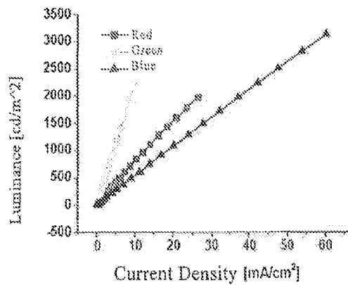
Fig. 6c (PRIOR ART)
